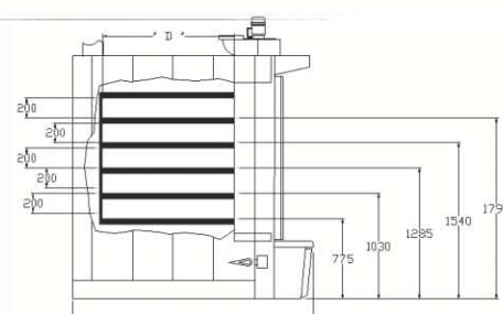
5 camere / 5 chambers
