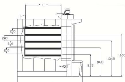
4 camere / 4 chambers
