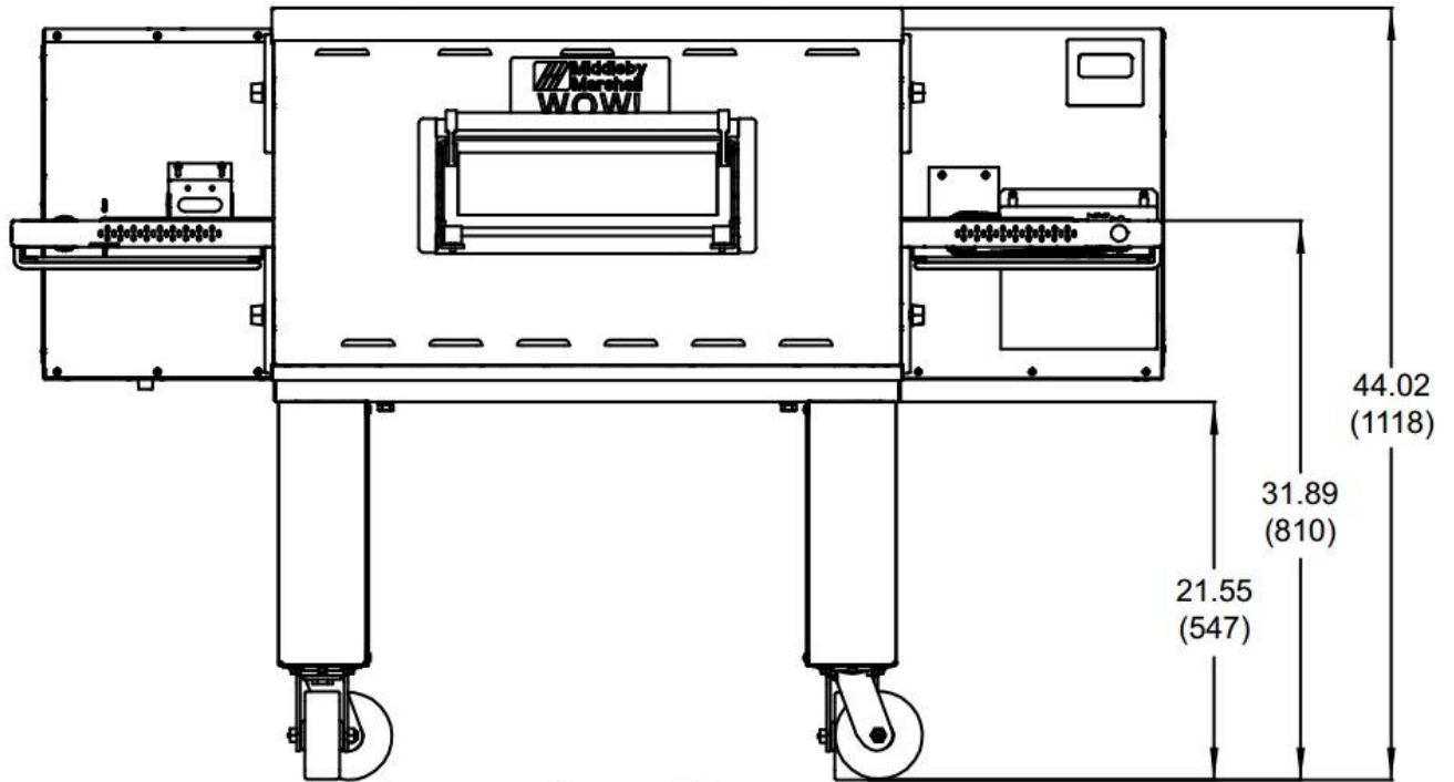
FRONT VIEW
