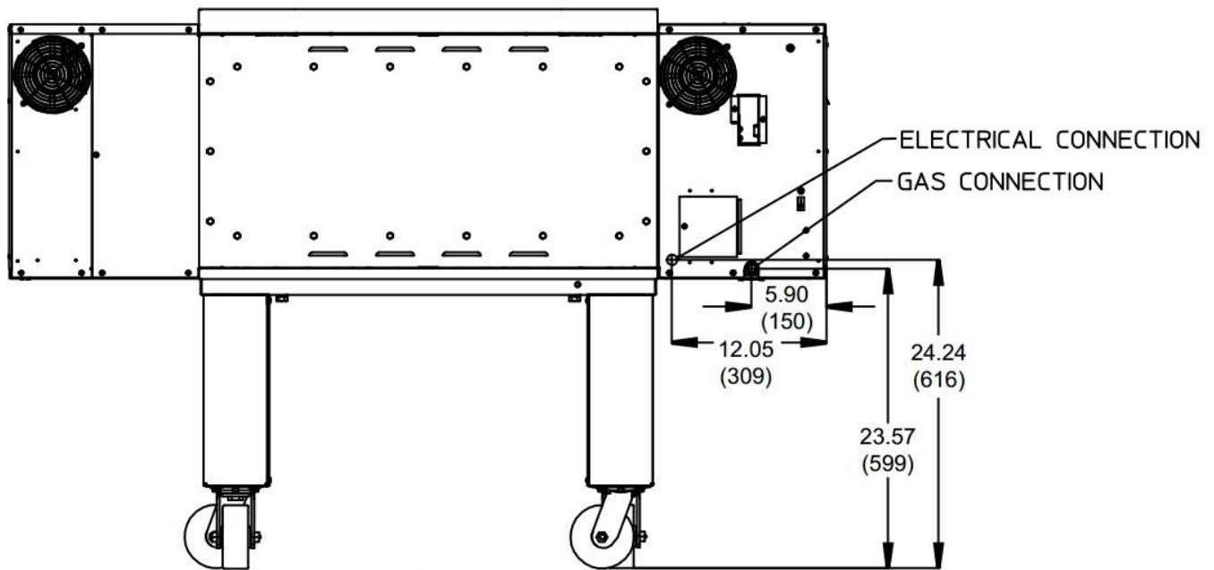
BACK VIEW
