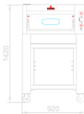
VISTA FRONTALE + SUPPORTO FRONT VIEW + STAND
